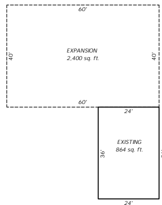
Maintenance Garage
